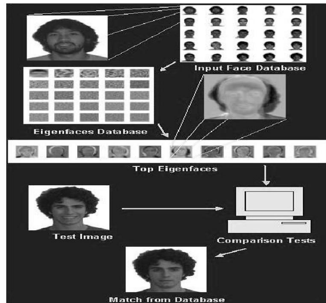
The Eigenface face recognition system segments.
