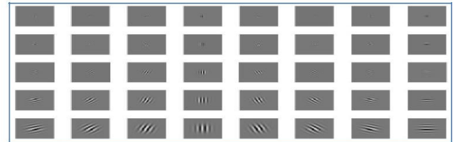
Gabor Filters
