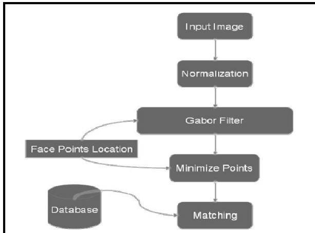
Normalize image
