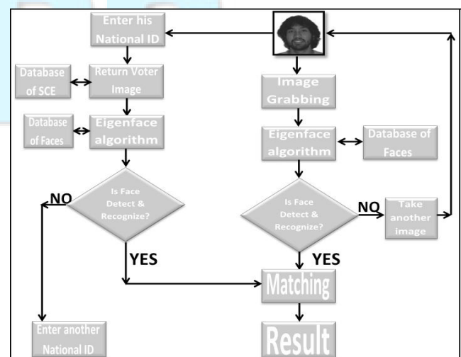
Online Voting System Based on Face Recognition using Eigenface system
